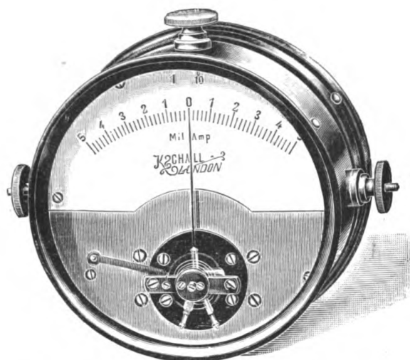
FIG. 44.—D'ARSONVAL GALVANOMETER.
