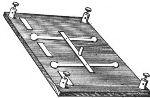
FIG. 50.—CURRENT REVERSER.
