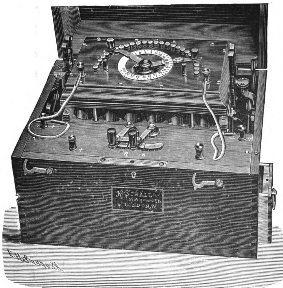
FIG. 94.—REINIGER'S BATTERY WITH AUTOMATIC PLUNGE APPARATUS.
