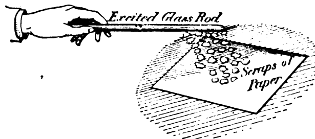
FIG. 1.—GLASS ROD AND SCRAPS OF PAPER.
