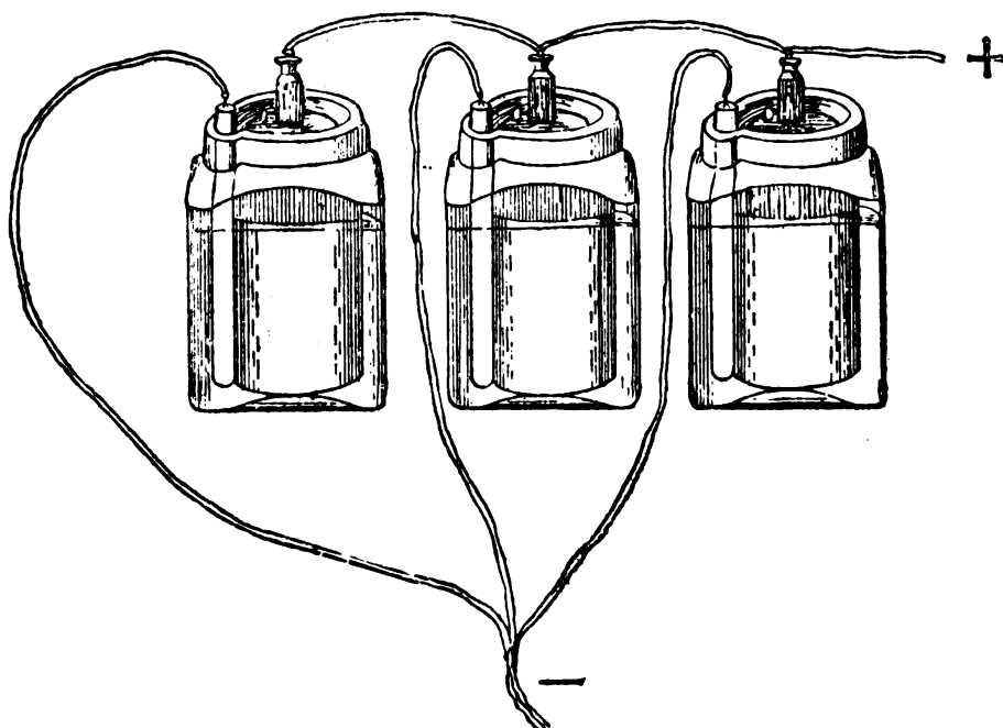
FIG. 30.—THREE CELLS IN PARALLEL.
