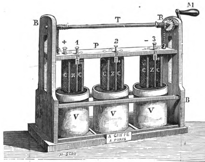
FIG. 18.—BICHROMATE BATTERY.
