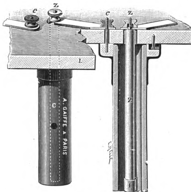
FIG. 20.—ARRANGEMENT OF ZINC AND CARBON.
