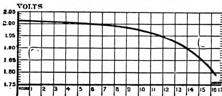
FIG. 84.—DRAKE AND GORHAM'S CURVE.
