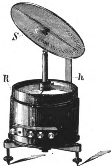
FIG. 42.—EDELMAUN'S GALVANOMETER.
