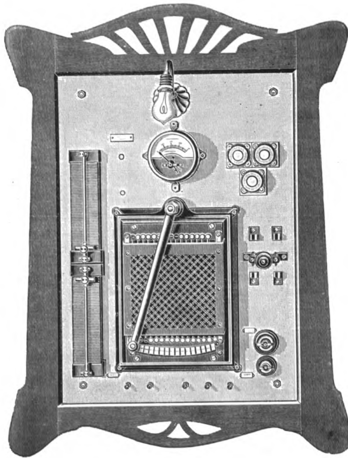
FIG. 191.—SWITCHBOARD FOR TRANSFORMER (Schall).
