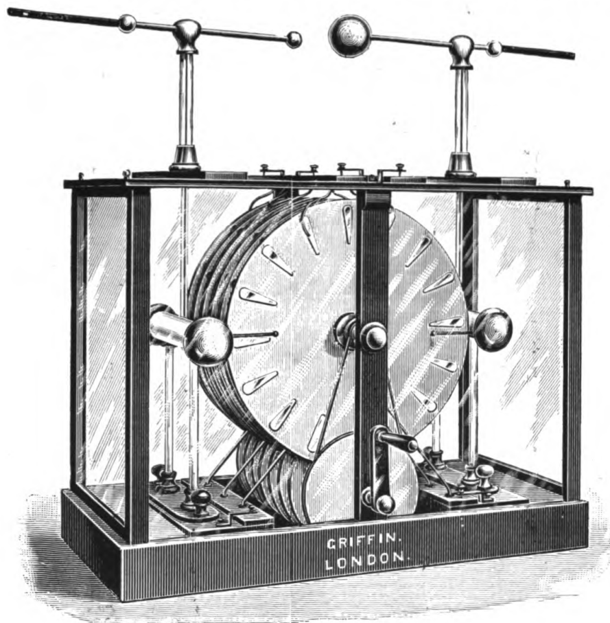
FIG. 6.—MULTIPLATE INFLUENCE MACHINE.
