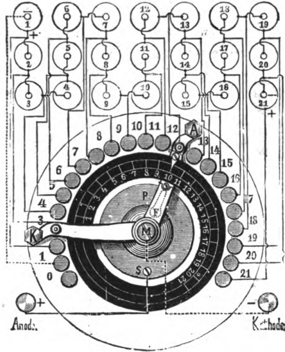
FIG. 49.—CONNECTIONS OF DOUBLE COLLECTOR.
