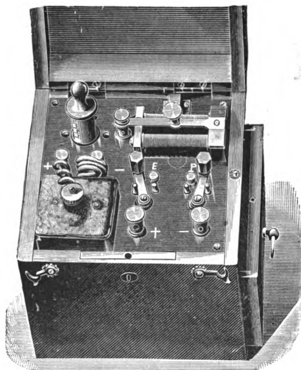
FIG. 93.—INDUCTION COIL WITH DRY CELL.
