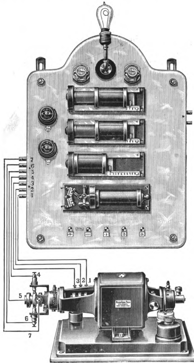
FIG. 74.—SINGLE PHASE OR THREE PHASE SINUSOIDAL MOTOR.
