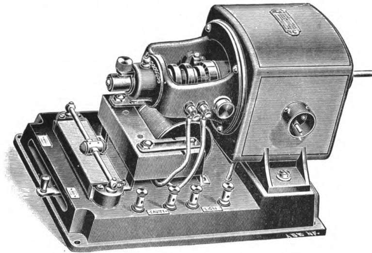
FIG 75.—MOTOR TRANSFORMER FOR LIGHT, CAUTERY, AND SINUSOIDAL TREATMENT.
