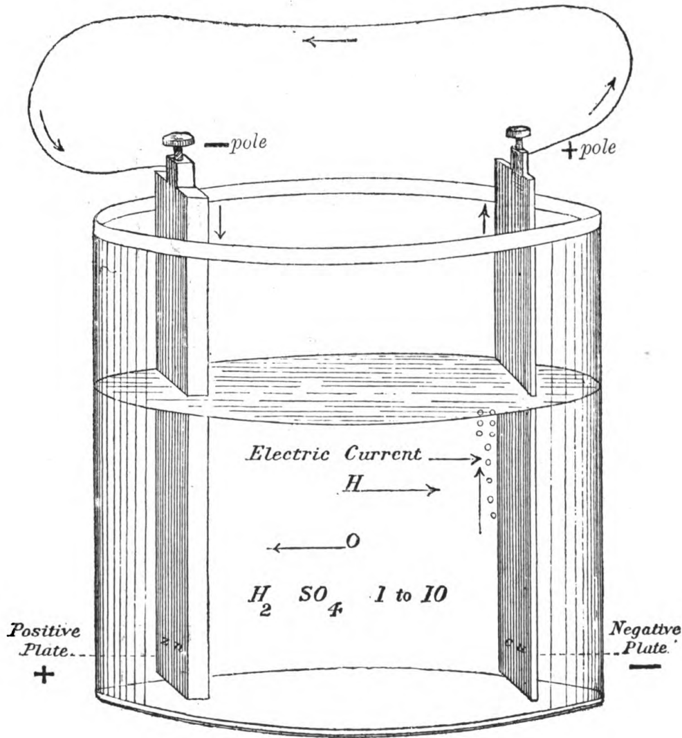
FIG. 12.—SIMPLE CELL.
