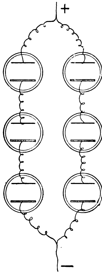
FIG. 32.—SIX CELLS IN COMPOUND CONNECTION.
