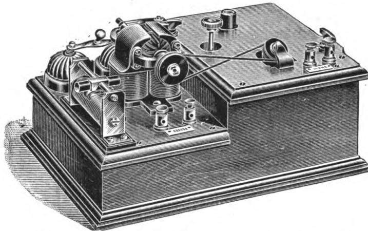
FIG. 141.—MACKENZIE-DAVIDSON INTERRUPTER. ]
