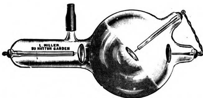
FIG. 159.—X-RAY TUBE PROPERLY EXCITED.
