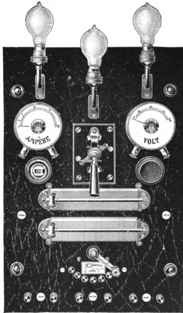
FIG. 150.—RESISTANCE FOR WORKING COILS FROM MAINS.
