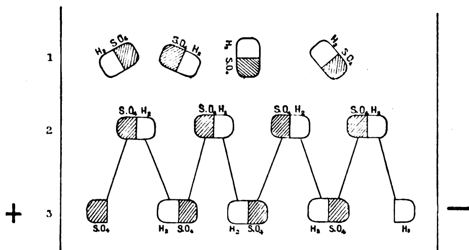
FIG. 99.—THEORY OF ELECTROLYSIS.
