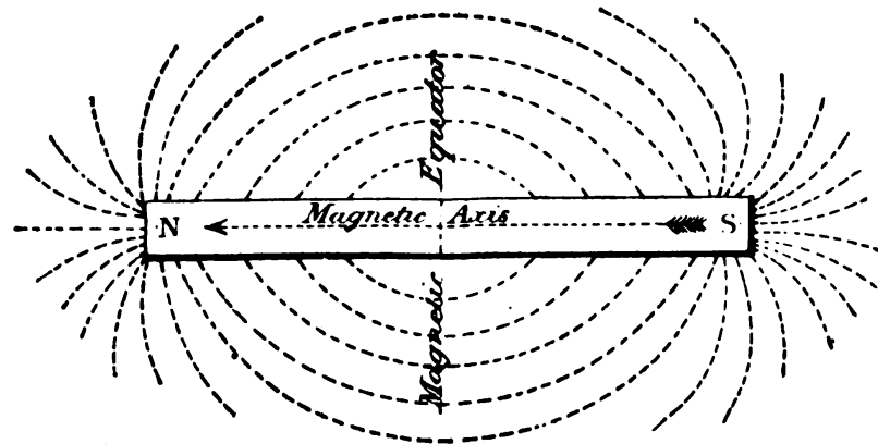
FIG. 8.—DIAGRAM OF A BAR MAGNET.
