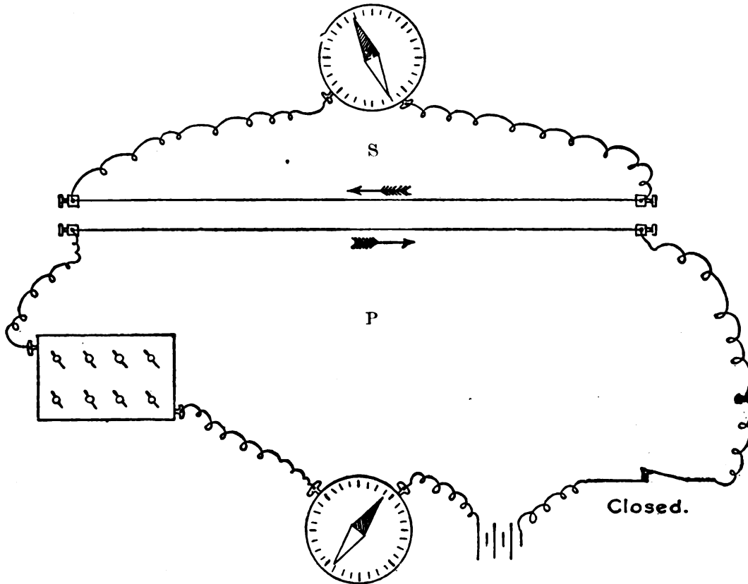
FIG. 65.—CURRENT IN OPPOSITE DIRECTION AT CLOSING.
