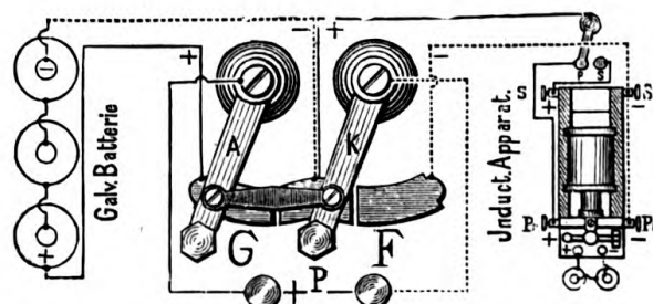
FIG. 60.—DIAGRAM OF CONNECTIONS OF DE WATTEVILLE'S KEY.
