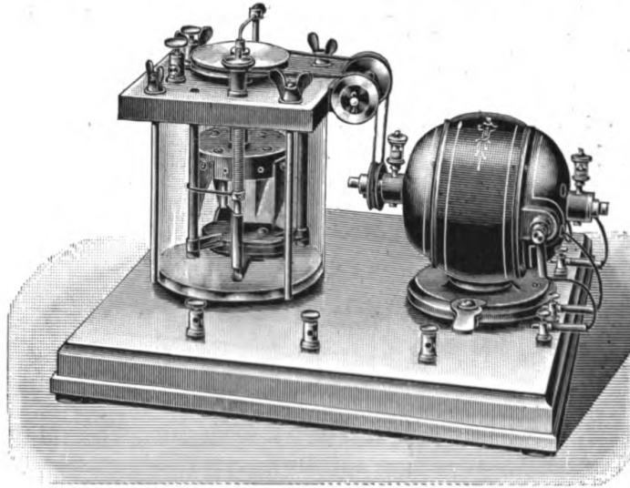
FIG. 142.—MERCURY JET INTERRUPTER.
