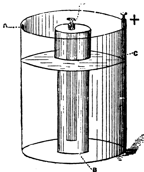
FIG. 22.—DANIELL CELL.
