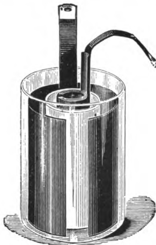
FIG. 23.—DANIELL CELL.
