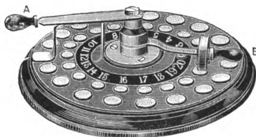
FIG. 47.—DOUBLE COLLECTOR.
