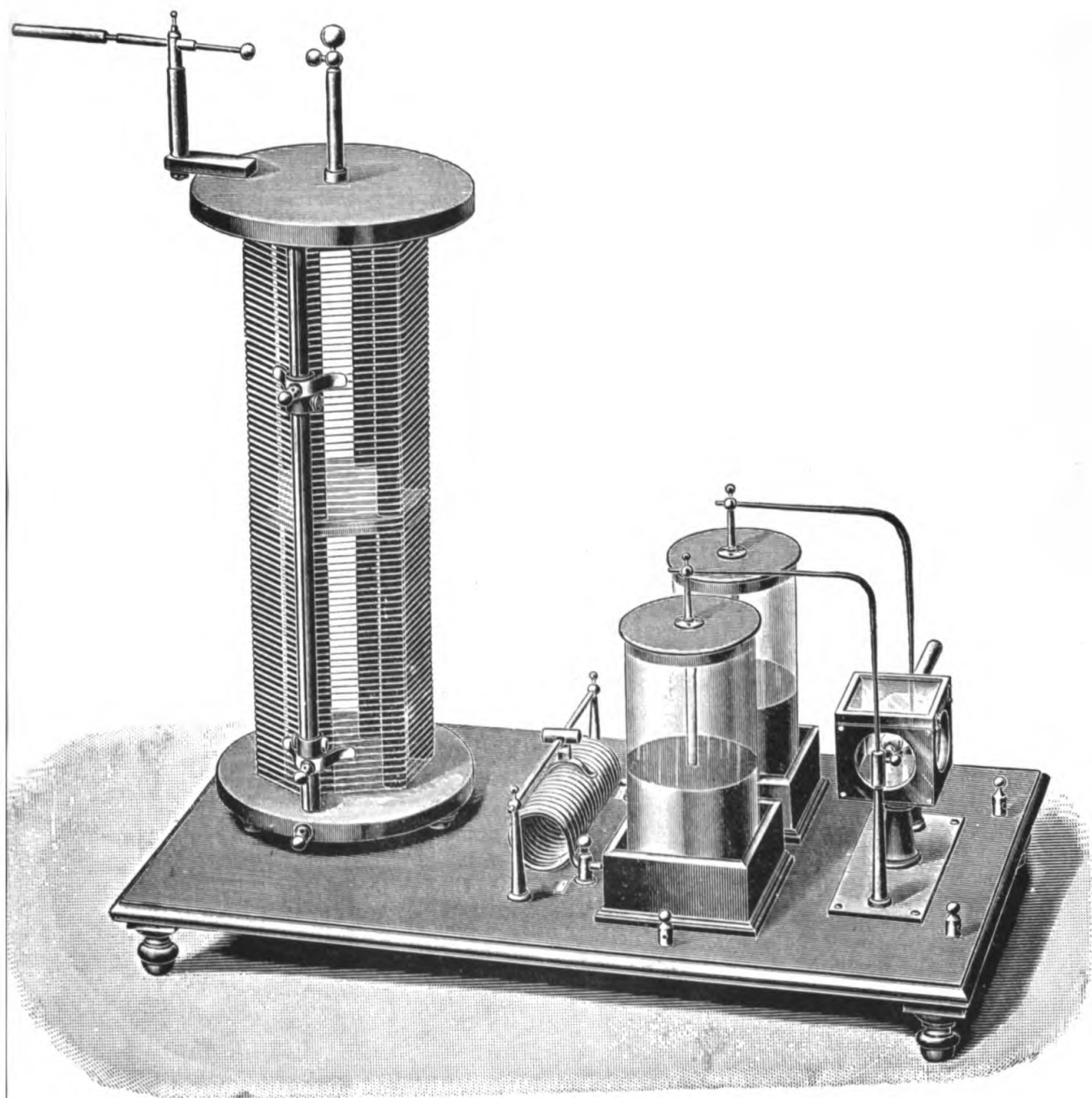
FIG. 195.—OUDIN'S RESONATOR AND SOLENOID.
