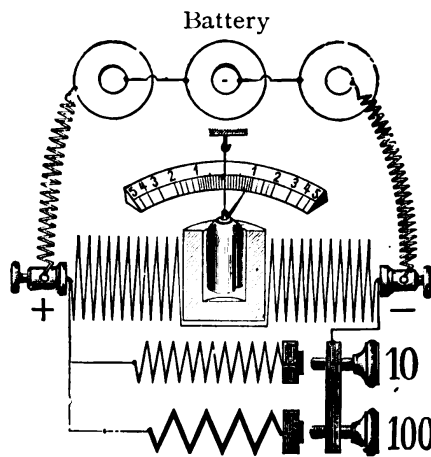
FIG. 41.—GALVANOMETER SHUNTS.
