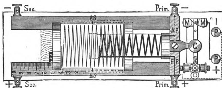
FIG. 69.—DIAGRAM OF INDUCTION COIL FROM ABOVE.
