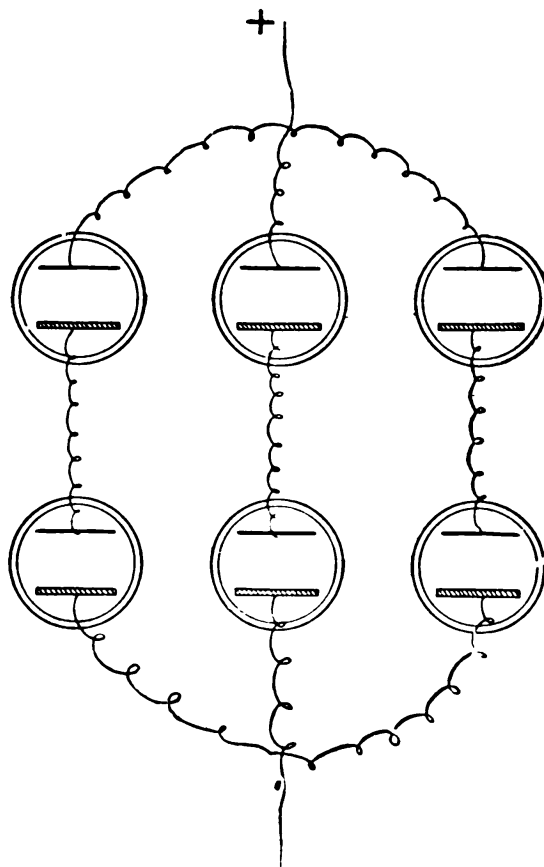
FIG. 33.—SIX CELLS IN COMPOUND CONNECTION.
