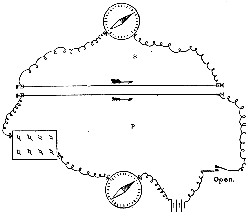
FIG. 66.—CURRENT IN SAME DIRECTION AT OPENING.
