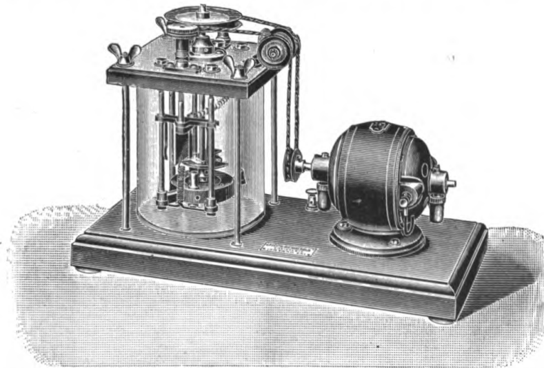
FIG. 143.—MERCURY JET INTERRUPTER. (LATER FORM.)
