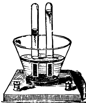
FIG. 98.—ELECTROLYSIS APPARATUS.
