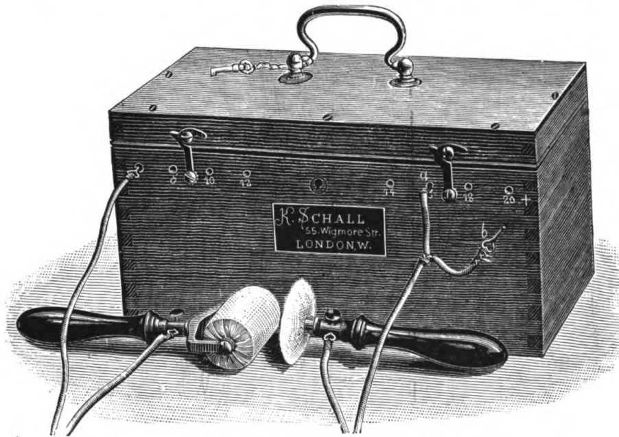
FIG. 45.—BATTERY WITH PLUG COLLECTOR.
