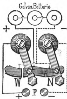
FIG. 51.—CONNECTIONS OF CURRENT REVERSER.
