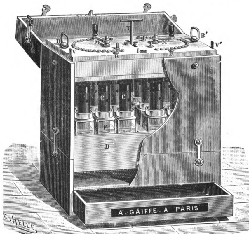
FIG. 19.—PERSULPHATE OF MERCURY CELL BATTERY.
