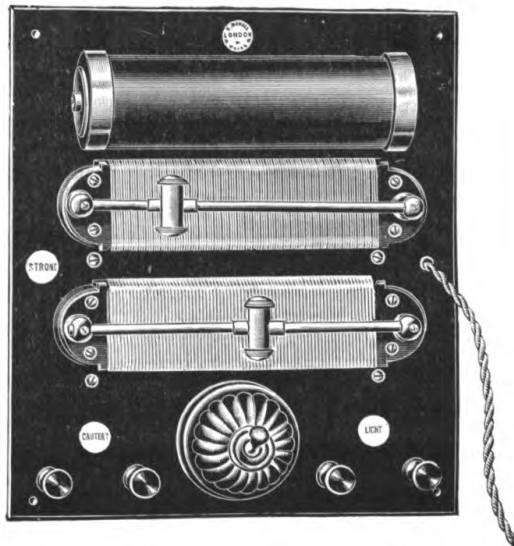
FIG. 81.—SIMPLE CURRENT TRANSFORMER.
