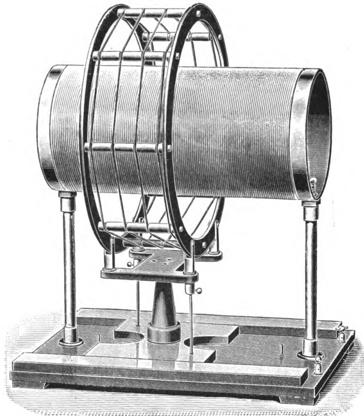
FIG. 194.—D'ARSONVAL'S BIPOLAR TRANSFORMER.
