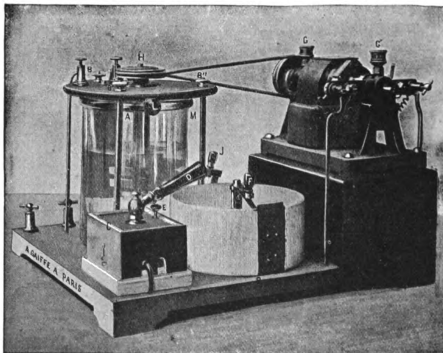
FIG. 148.—THE CONTREMOULINS-GAIFFE INTERRUPTER.
