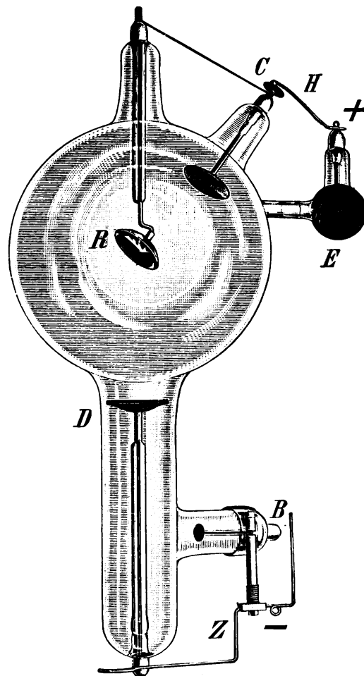
FIG. 154.—HIRSCHMANN'S TUBE, WITH REGULATING ARRANGEMENT.
