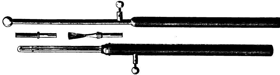
FIG. 196.—HIGH-FREQUENCY ELECTRODES.
