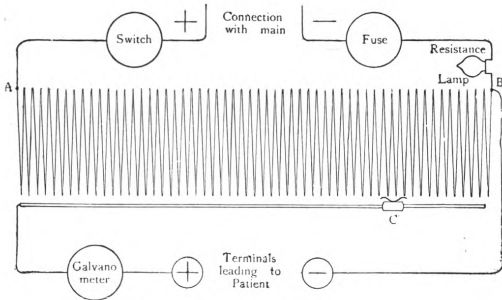
FIG. 77.—PORTABLE SWITCH-BOARD.
