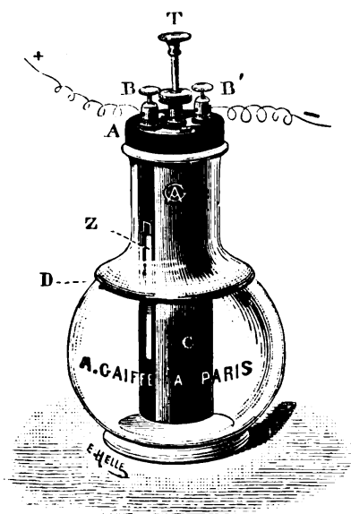
FIG. 17.—BOTTLE BICHROMATE CELL.
