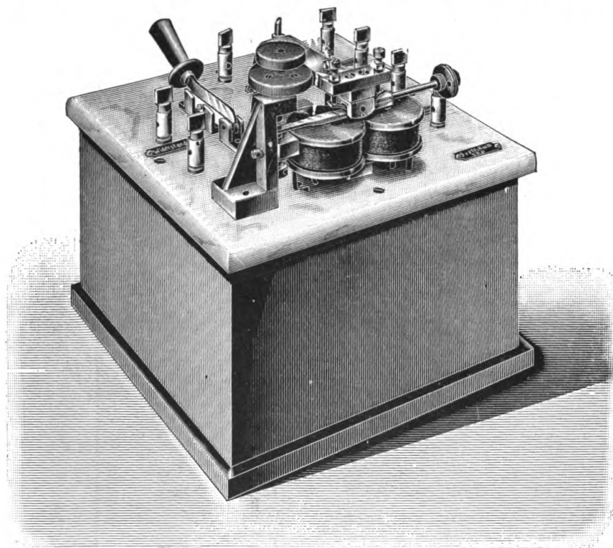
FIG. 151.—ALTERNATING CURRENT RECTIFIER.
