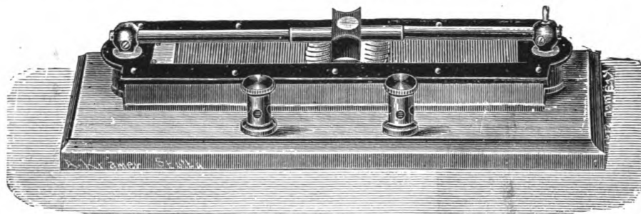
FIG. 149.—ADJUSTABLE RESISTANCE.
