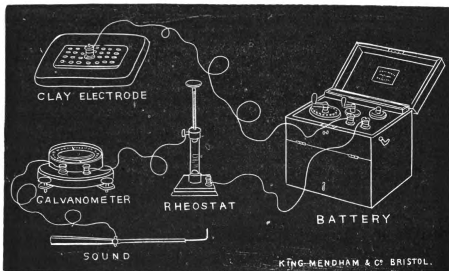
FIG. 126.—ARRANGEMENT OF APPARATUS FOR THE APOSTOLI TREATMENT.
