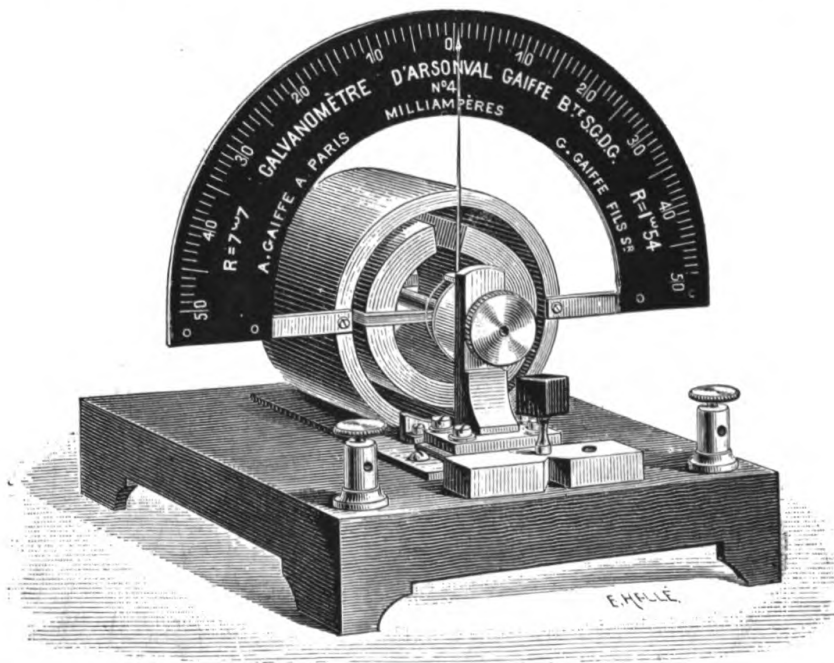
FIG. 43.—D'ARSONVAL'S GALVANOMETER WITH VERTICAL SCALE.
