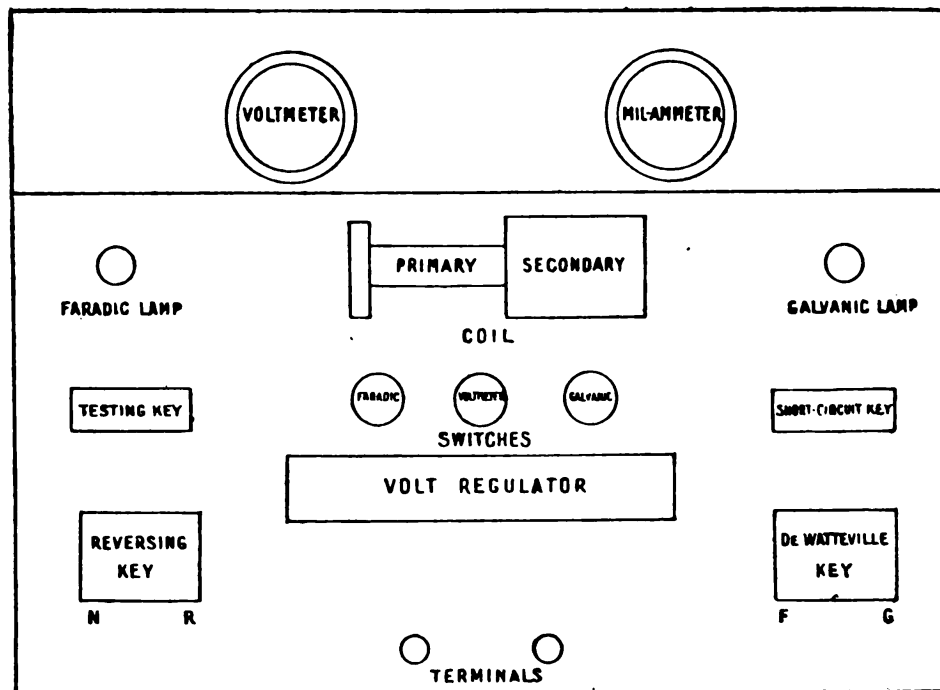
FIG. 80.—DIAGRAM OF ARRANGEMENT OF MILNE MURRAY'S SWITCH-BOARD.
