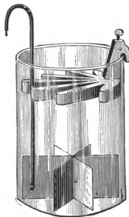
FIG. 24.—GRAVITY CELL.
