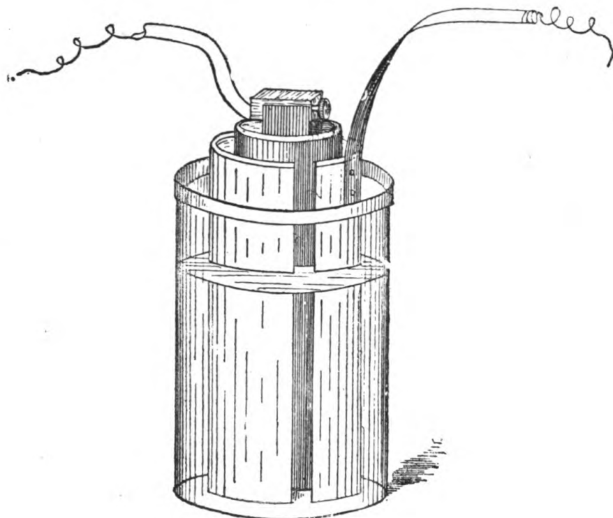
FIG. 25.—BUNSEN CELL.
