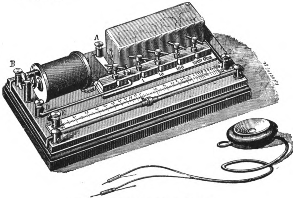
FIG. 29.—KOHLEAUSCH'S BRIDGE.
