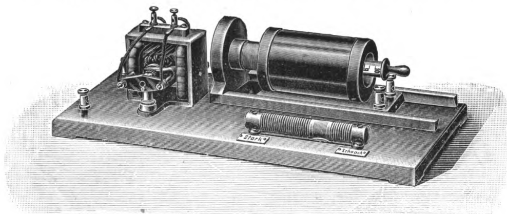
FIG. 73.—SINGLE PHASE SINUSOIDAL MOTOR.
