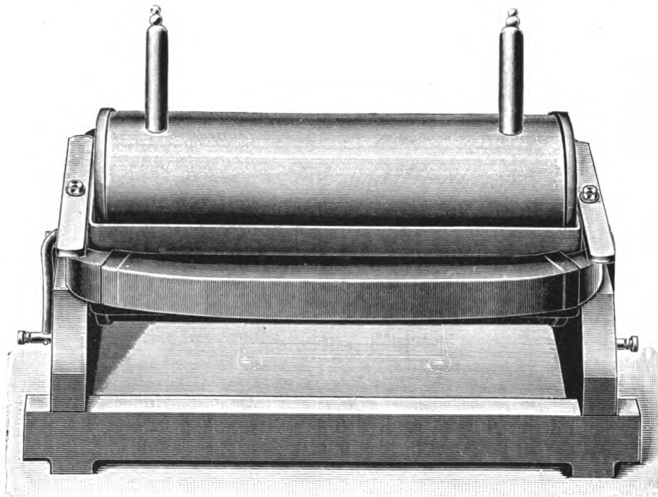
FIG. 195.—CLOSED IRON CIRCUIT TRANSFORMER (Schall).
