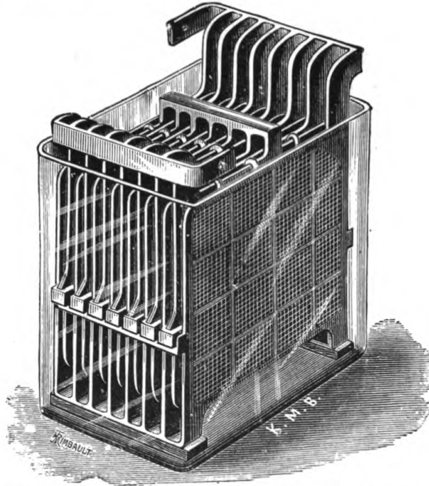
FIG. 83.—ACCUMULATOR IN GLASS VESSEL.
