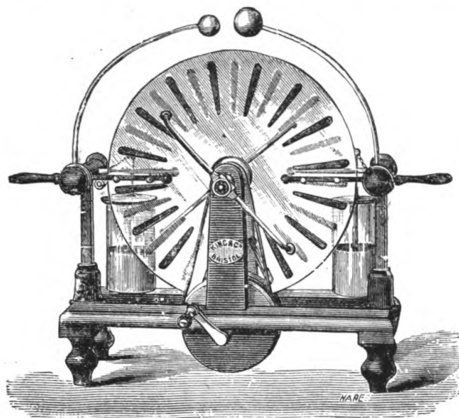
FIG. 5.—WIMSHURST MACHINE.
