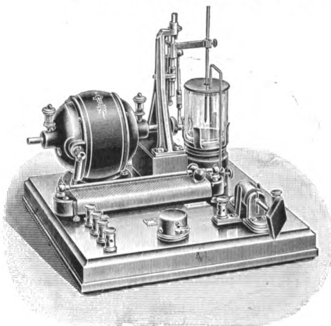
FIG. 140.—DIPPING INTERRUPTER.
