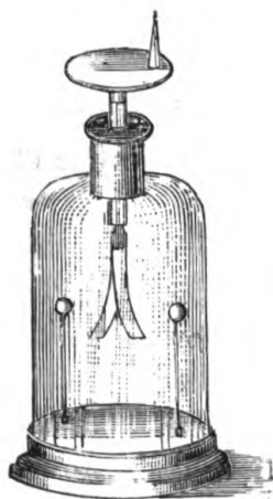
FIG. 3.—ELECTROSCOPE.
