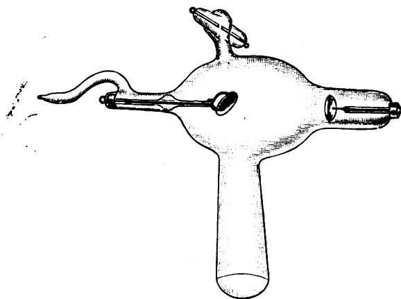
FIG. 160A.—THERAPEUTIC TUBE.
