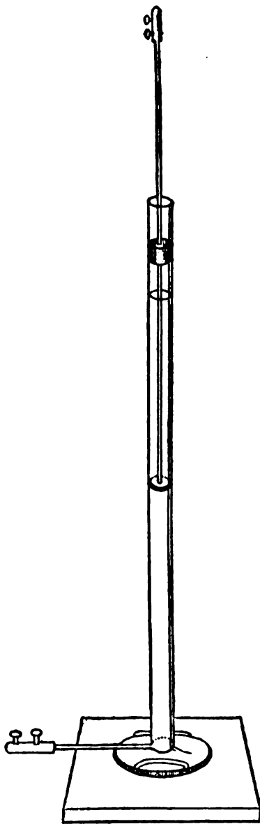
FIG. 56.—ORDINARY LIQUID RHEOSTAT.
