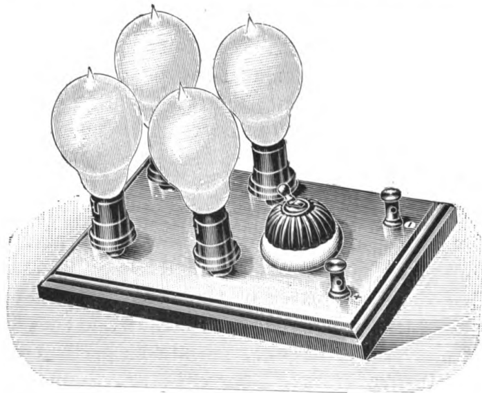
FIG. 86.—LAMPS IN PARALLEL FOR CHARGING AN ACCUMULATOR.
