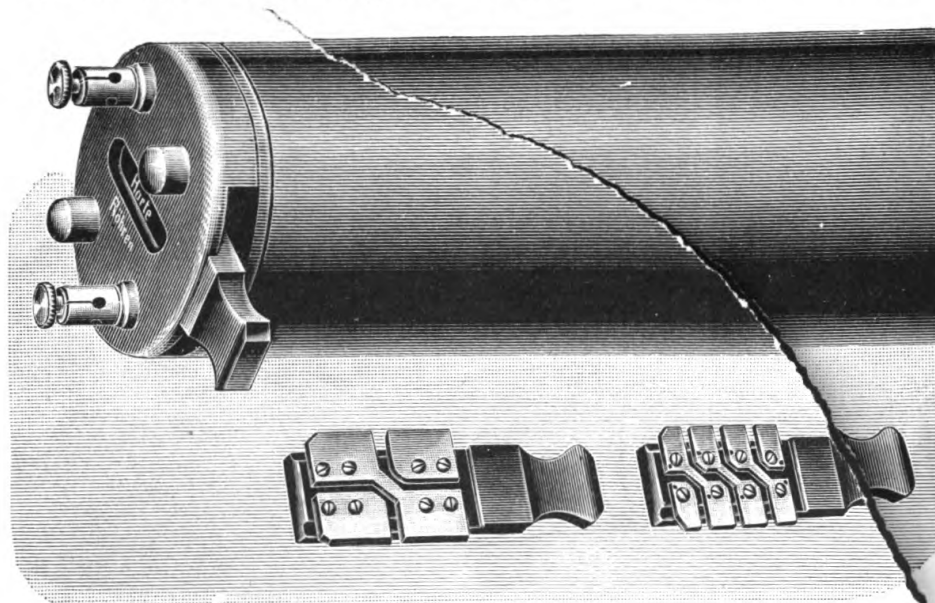
FIG. 157.—COIL WITH ADJUSTABLE SELF-INDUCTION.
