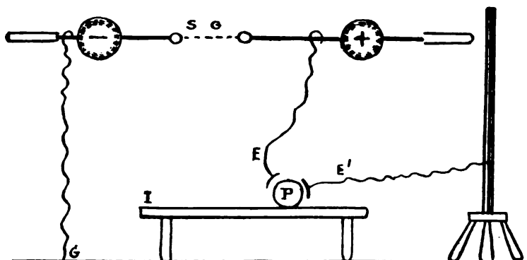
Fig. 42.—The wave-current intensified. (Morton.)
