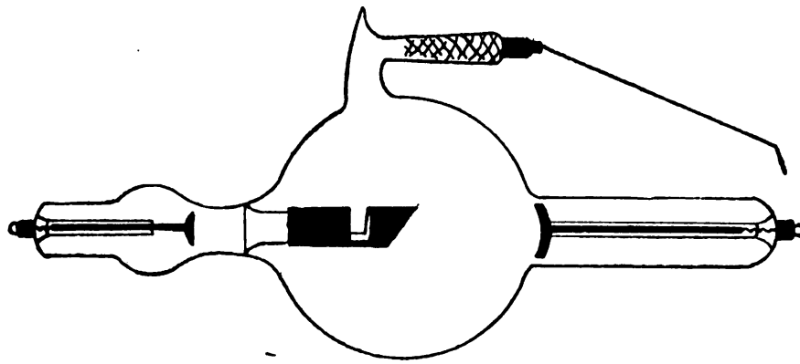
Fig. 66.—Campbell X-ray tube.
