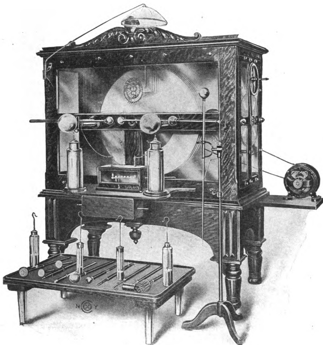
Fig. 37.—Waite and Bartlett's static machine.
