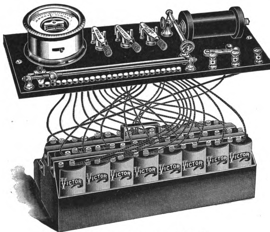
Fig. 5.—Removable tray. (Victor.)
