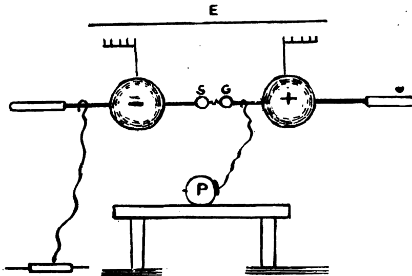
Fig. 41.—Wave-current. (Morton.)
