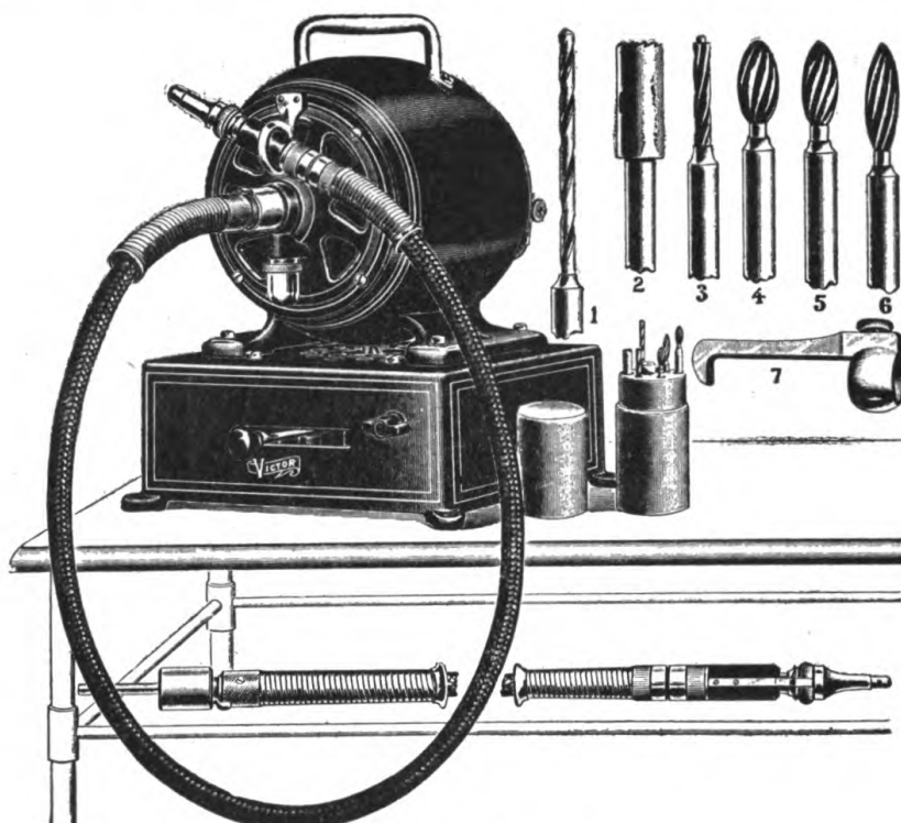
Fig. 55.—Victor bone engine.
