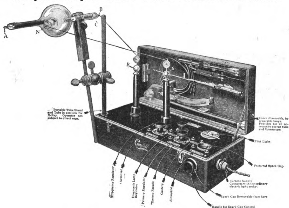
Fig. 74.—Campbell model "E" X-ray and coil.
