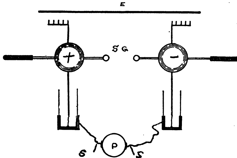
Fig. 61.—Drawing of Morton's static induced current of 1881.
