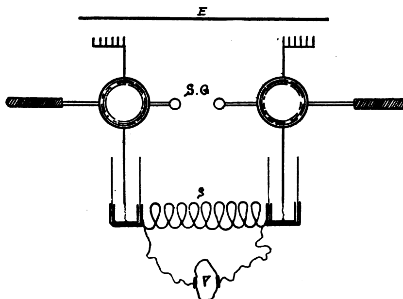
Fig. 63.—Drawing of d'Arsonval apparatus.
