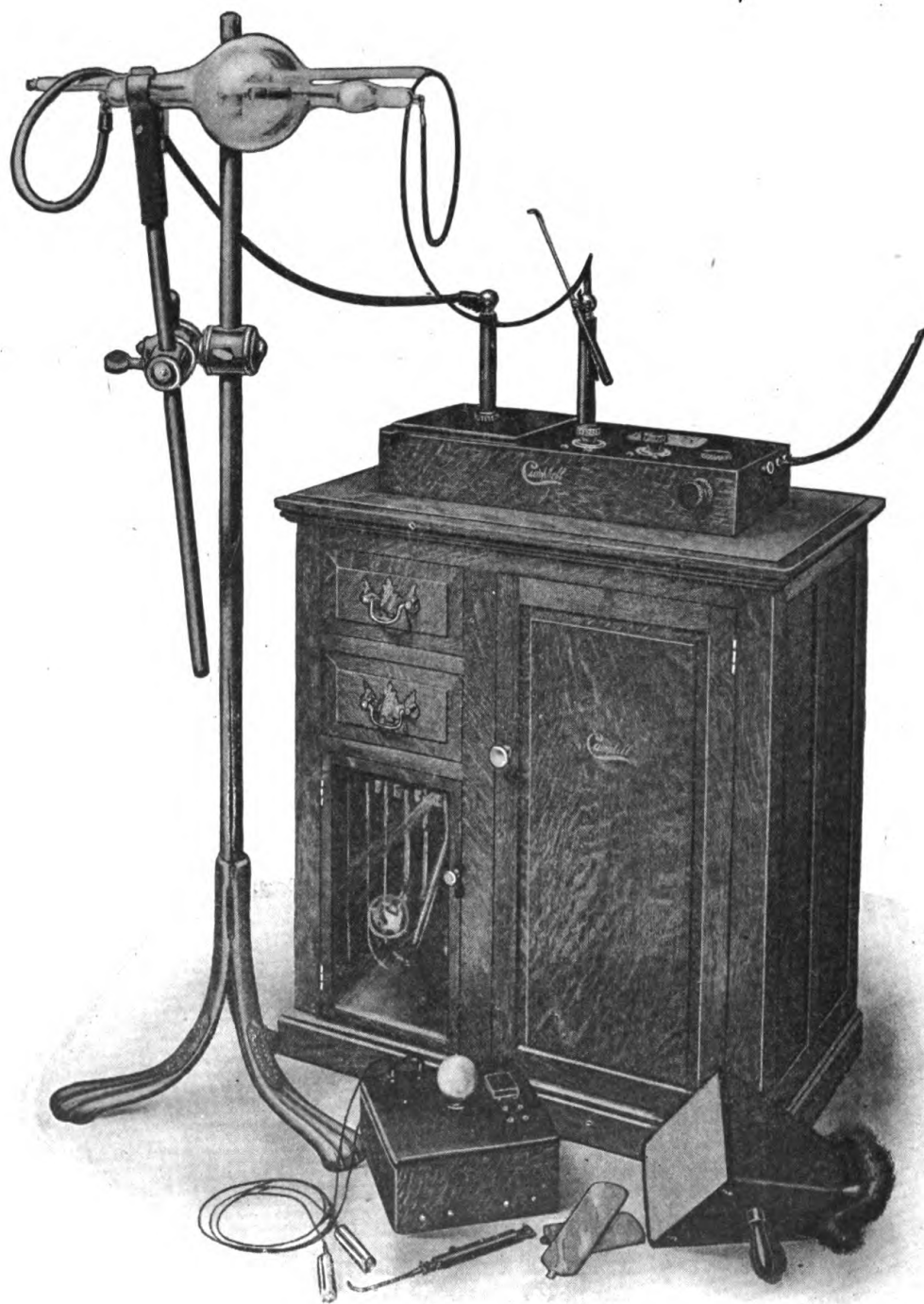
Fig. 71.—Campbell model "D" coil, cabinet and X-ray.
