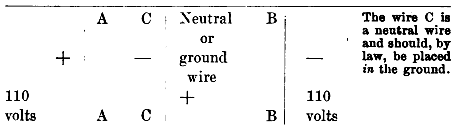
Fig. 9.—Diagram of three-wire system.
