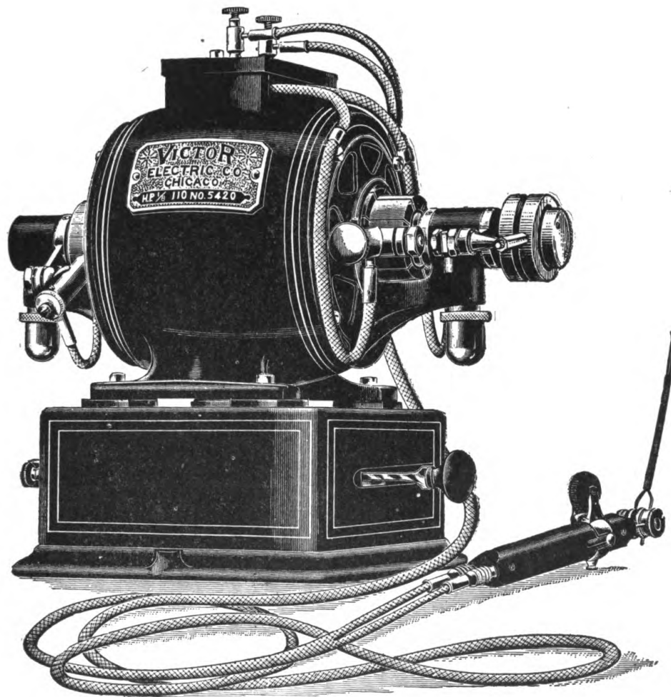
Fig. 60.—Victor No. 9 transformer.
