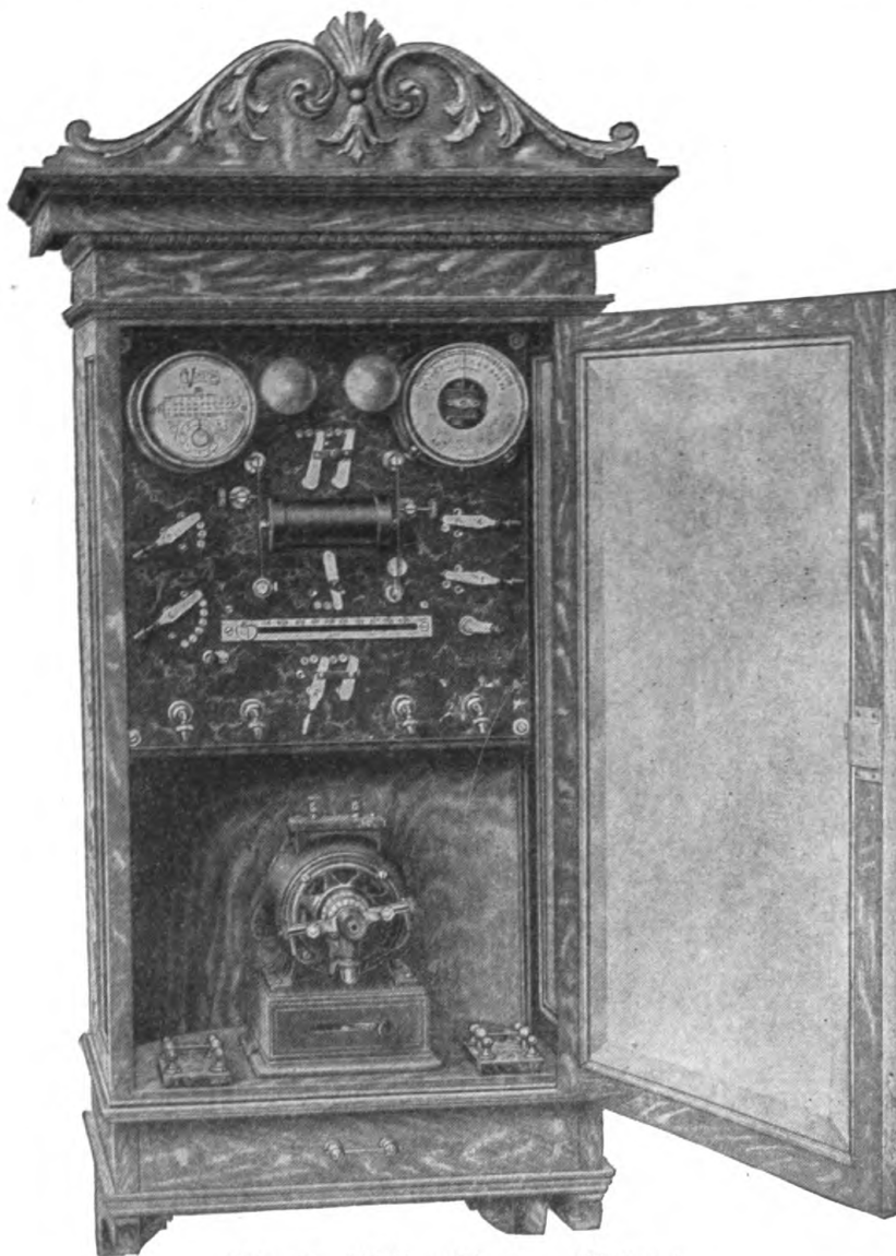
Fig. 7.—Wall cabinet. (Victor.)
