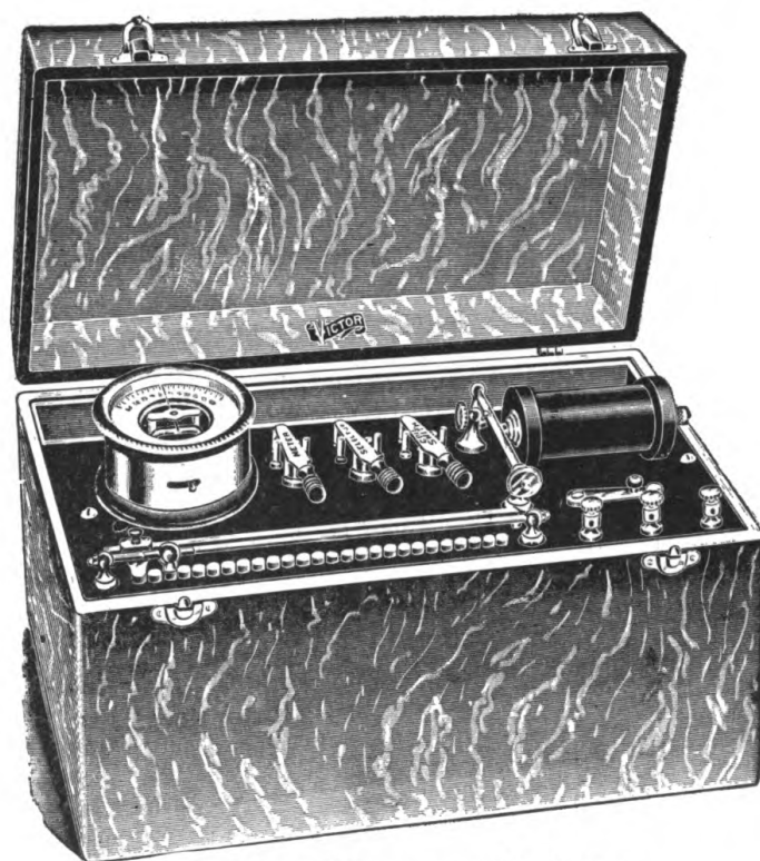
Fig. 4.—No. 5 Victor portable battery.
