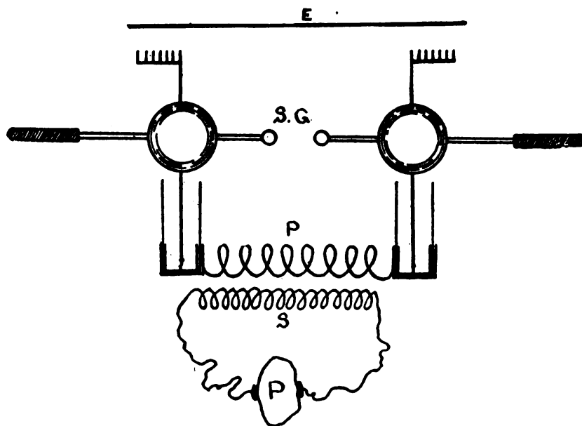
Fig. 64.—Drawing of Tesla apparatus.
