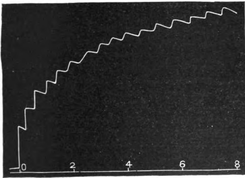
FIG. 116. Multiple Mechanical Response of Biophytum , due to a Single Thermal Stimulus
