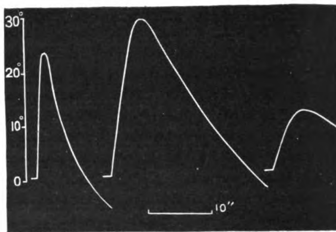
FIG. 33. Response of Leaves of Ordinary Plants to Electric Stimulation The ordinate represents the angular movement in degrees.
