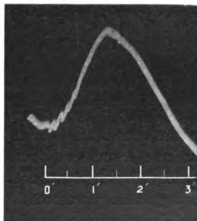
FIG. 126. Photographic Record of Pulsation of Desmodium
