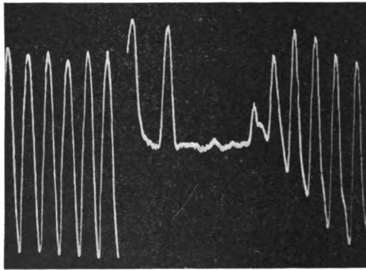
FIG. 141. Effect of Rapid Cooling by Ice-cold Water
