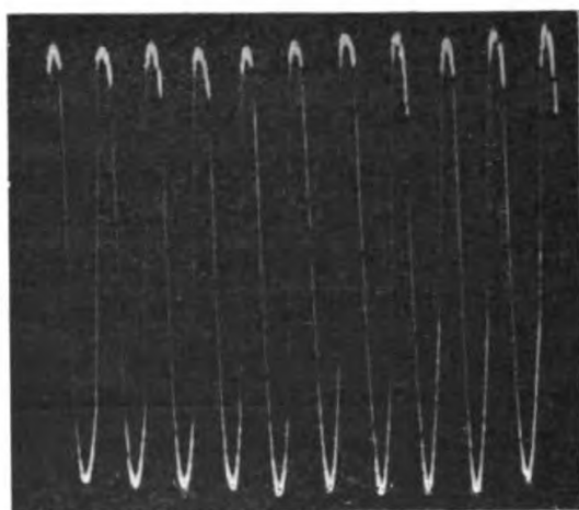
FIG. 127. Photographic Record of Uniform Pulsations in Desmodium
