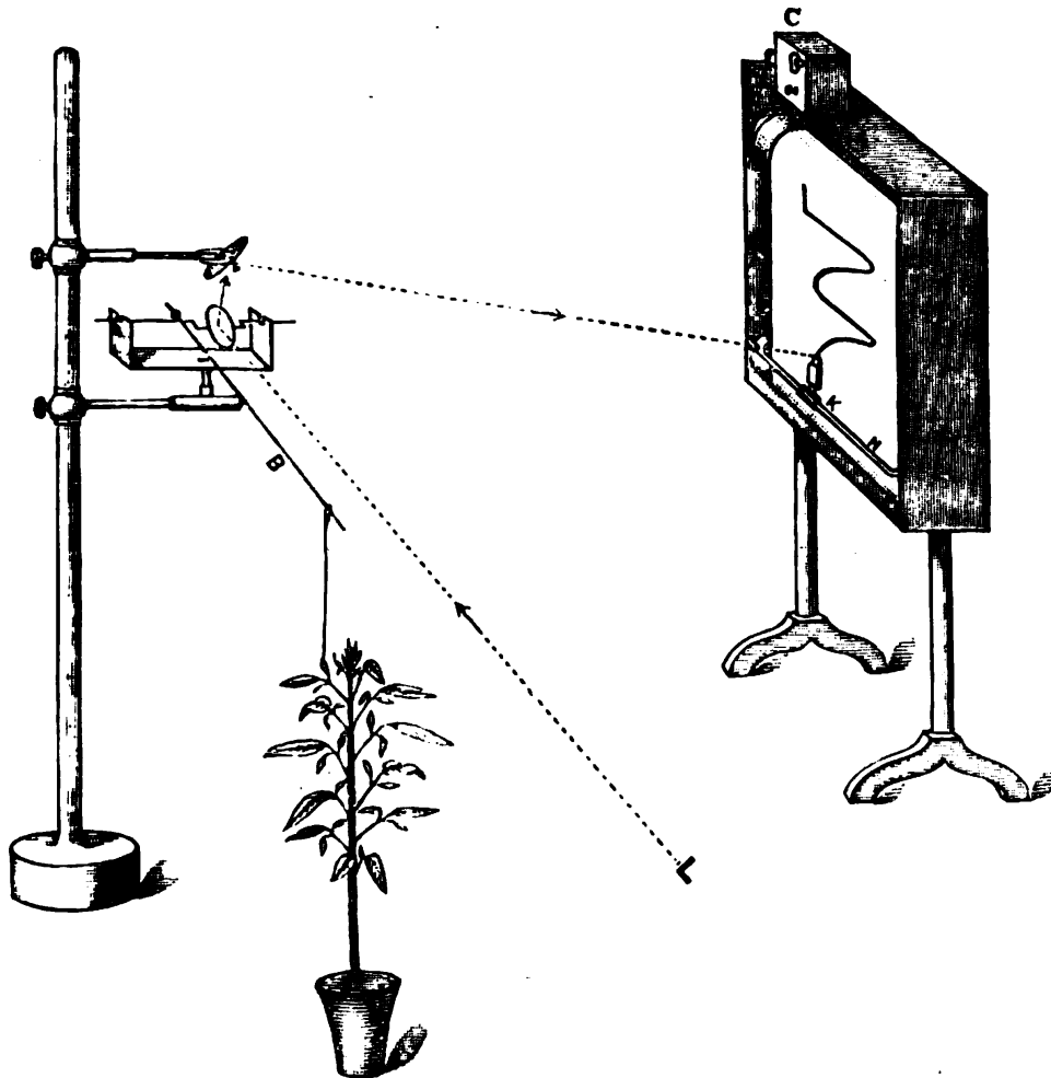
FIG. 4. Demonstration Optical Pulse-Recorder
