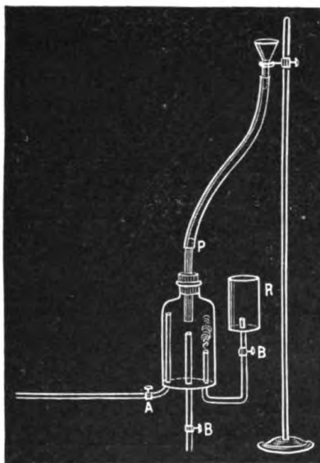
FIG. 160. Method of Hydrostatic Balance
