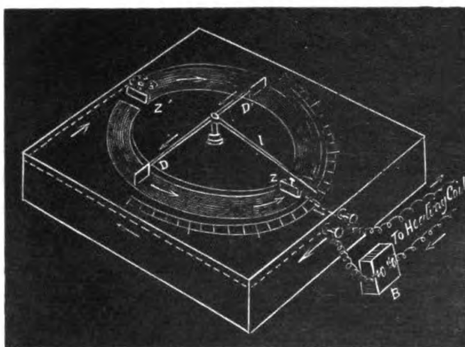
FIG. 181. Semicircular Electrolytic Rheostat interposed in Heating Coil
