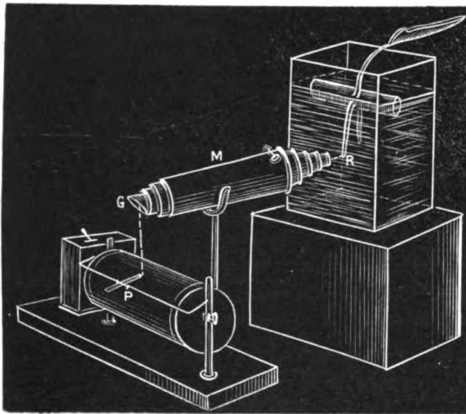
FIG. 244. Microscope Recorder
