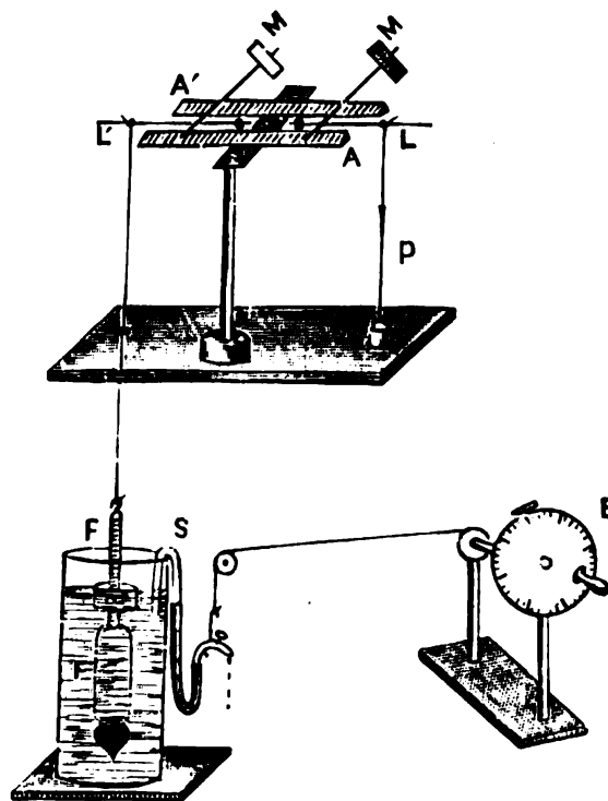
FIG. 167. Diagrammatic Representation of Balanced Crescograph
