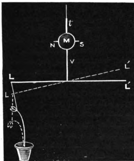
FIG. 240. Diagrammatic Representation of the Magnetically Controlled Recorder
