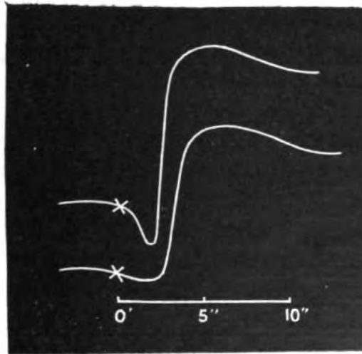
FIG. 27. The Abnormal Positive preceding the Normal Negative in Mechanical and Electrical Responses in Biophytum × represents the moment of application of stimulus. The upper is the mechanical and the lower the electrical record. The records downward indicate erection of the leaf or galvanometric positivity.
