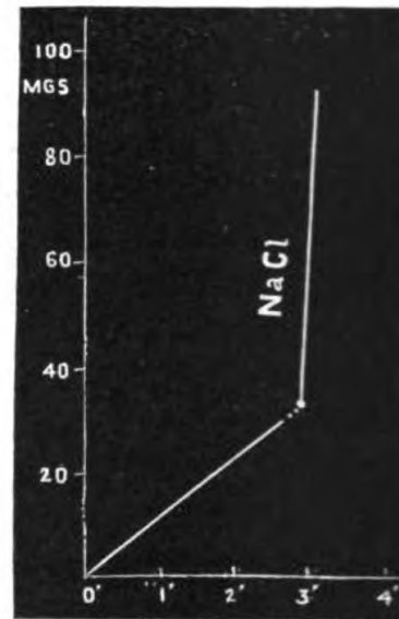
FIG. 164. Effect of Strong NaCl Solution
