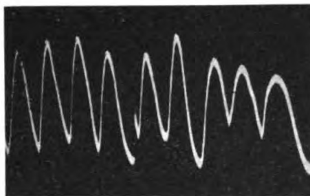
FIG. 151. Effect of Barium Chloride Solution on Desmodium
