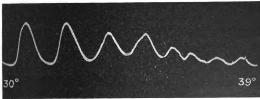
FIG. 137. Photographic Record of Pulsations of Desmodium during Continuous Rise of Temperature
