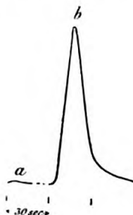
FIG. 45. Additive Effect in Electrical Response
