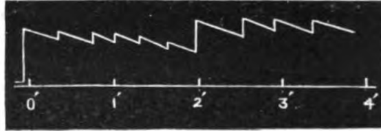
FIG. 119. Multiple Response in Biophytum , showing Cyclic Groupings of Amplitude and Period
