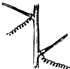
FIG. 90. Bi-polar Excitation of Mimosa
