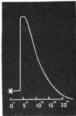
FIG. 107. Electrotactile Response in Stem of Mimosa
