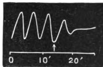
FIG. 6. Death, and Arrest of Pulsation, in Leaflet of Desmodium by Strong Electric Shock
