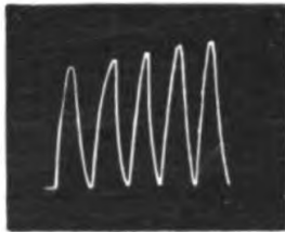
FIG. 52. Staircase Effect in Longitudinal Mechanical Response of Plant (Style of Eucharis )
