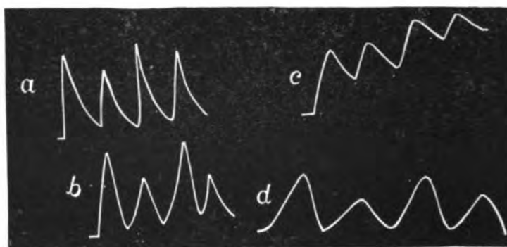
FIG. 55. Alternate Fatigue (a) in Electrical Responses of Petiole of Cauliflower ; (b) in Multiple Electric Responses of Peduncle of Biophytum ; (c) in Multiple Mechanical Responses of Leaflet of Biophytum ; and (d) in Autonomous Responses of Desmodium
