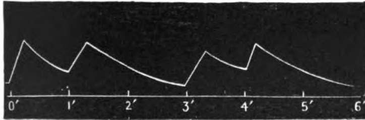
FIG. 122. Intermittence in Pulsation of Biophytum
