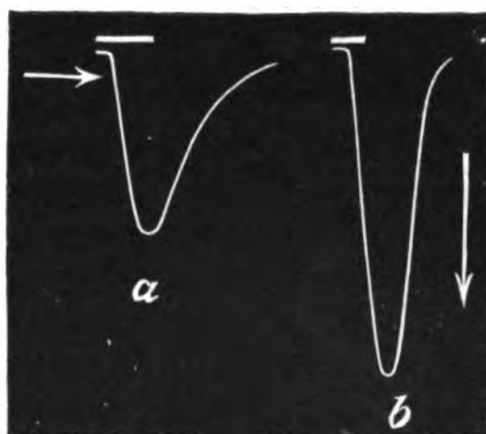
FIG. 257. Responses of Oxalis to Sunlight
