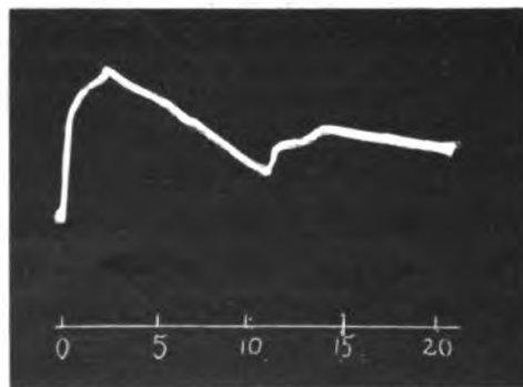
FIG. 58. Photographic Record of Periodic Fatigue under Continuous Stimulation in Contractile Response (Filament of Uriclis Lily)
