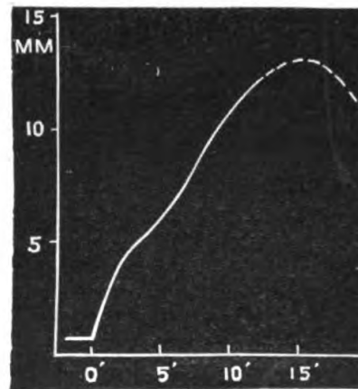
FIG. 243. Heliotropic Response of Sinapis to Sunlight
