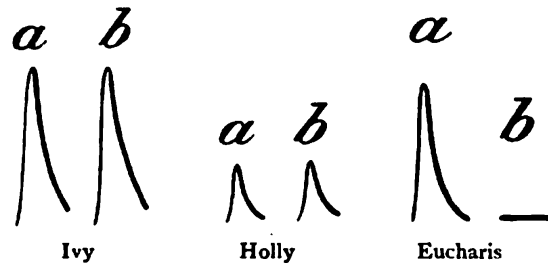
FIG. 76. After-effect of Cold on Ivy, Holly, and Eucharis (a) Normal response ; (b) response after subjection to freezing temperature for twenty-four hours.
