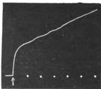
FIG. 195. Acceleration of Growth by Application of Solution of Sugar
