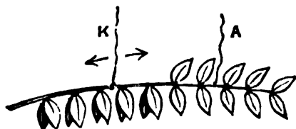
FIG. 91. Bi-polar Excitation of Biophytum
