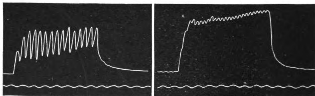
FIG. 49. Genesis of Tetanus in Muscle
