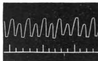
FIG. 150. Simple Alternation of Pulsation in Frog's Heart (Pembrey and Phillips)
