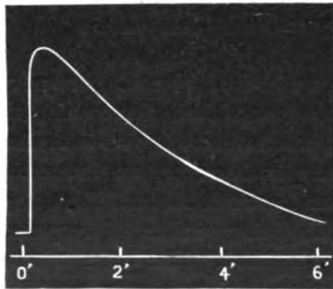
FIG. 21. Isometric Response of Mimosa
