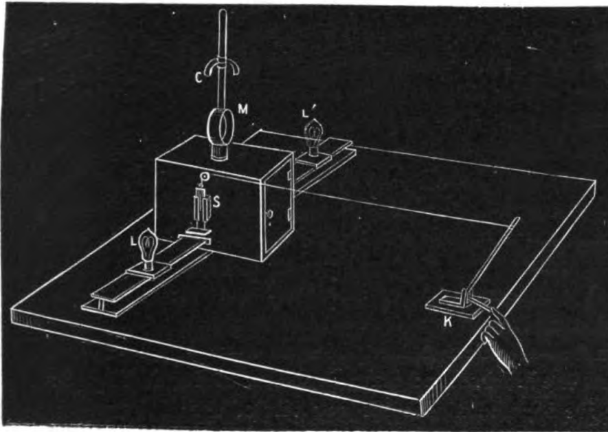
FIG. 241. Heliotropic Chamber and Magnetically Controlled Recorder
