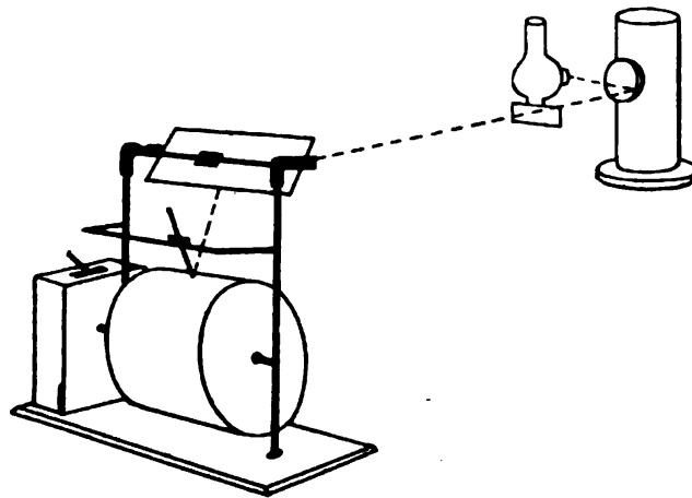
FIG. 24. Electric Response Recorder
