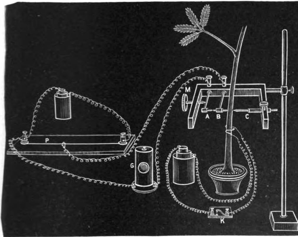
FIG. 106. Electrotactile Method for Detection of Excitatory Wave during Transit
