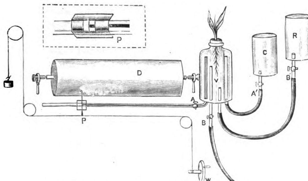
FIG. 156. Diagrammatic Representation of the Shoshungraph
