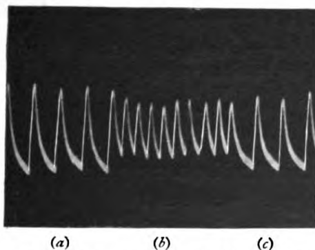
FIG. 54. Fatigue shown in Electrical Response, when sufficient Time is not allowed for Full Recovery
