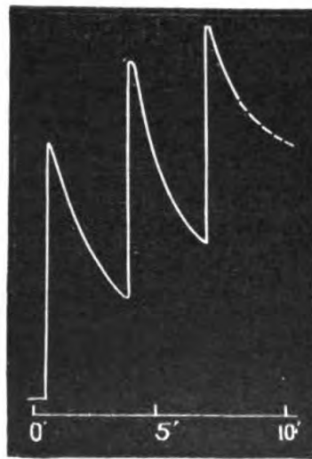
FIG. 123. Multiple Response of Biophytum under the Continuous Action of Light
