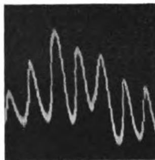
FIG. 143. Photographic Record of Cyclic Groupings in Autonomous Pulsations of Desmodium , showing Sub-pulses
