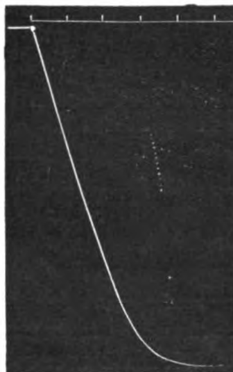
FIG. 217. Record showing Positive Electrical Variation indicating Positive Turgidity-Variation of Distal Point, under Moderate Stimulation of Proximal
