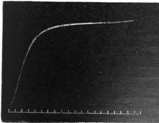
FIG. 16. Photographic Record of Response in different specimen, taken on a faster-moving drum, showing only first part of the curve. Each division of time-scale = \frac{1}{5} second.
