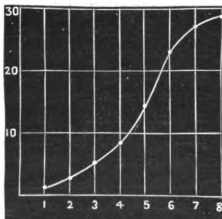
FIG. 47. Curve showing Relation between Stimulus and Response
