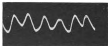
FIG. 149. Periodic Groupings of Pulsation in Desmodium
