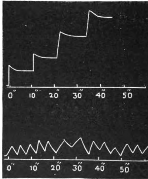
FIG. 176. Growth-pulsation seen in Seedling of Balsam
