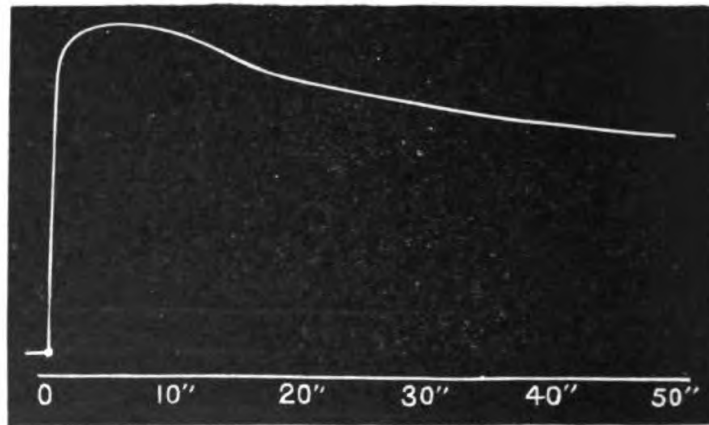
FIG. 112. Response of Biophytum ; Electrical Stimulus having been Applied at the Pulvinus of the Motile Leaflet The thick dot represents the moment of stimulation.
