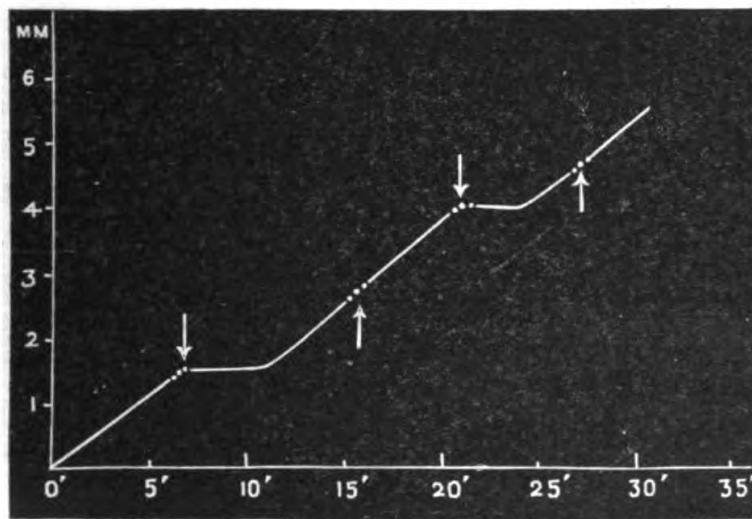
FIG. 211. Effect on Apogeotropic Movement of Temporary Applications of Cold alternately to Upper (↓) and Lower (↑) Surfaces of Horizontally laid Scape of Uriclis Lily
