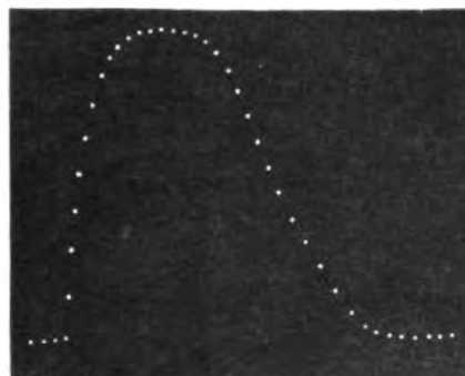
FIG. 134. Spark-record of Single Pulsation in Leaflet of Desmodium
