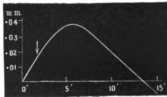
FIG. 250. Effect of Electric Waves on Growth
