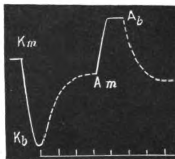
FIG. 231. Effects of Anode and Kathode on Variation of Rate of Growth in Root of Bindweed exhibited by Balanced Growth-record
