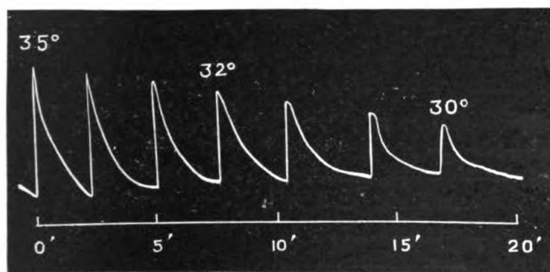
FIG. 124. Induction of Autonomous Response in Biophytum , at Moderately High Temperature of 35^{\circ} C.
