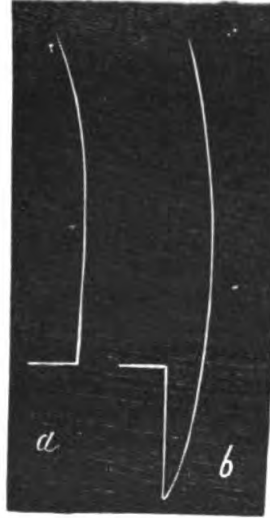
FIG. 224. Mechanical Responses of Leaf of Mimosa
