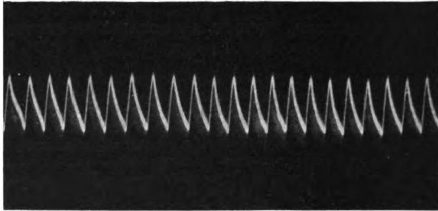
FIG. 51. Uniform Electrical Responses (Radish)
