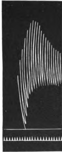
FIG. 65. Preliminary Staircase, followed by Fatigue, in the Responses of Muscle (Brodie)
