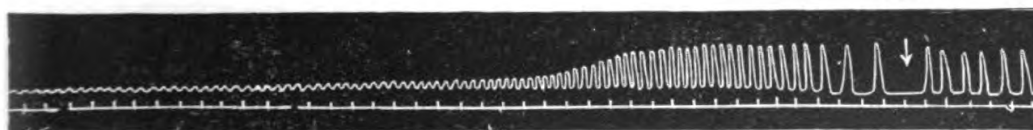
FIG. 152. Arrest of Beat of Ventricle of Frog at Diastole by Application of Acid at Arrow
