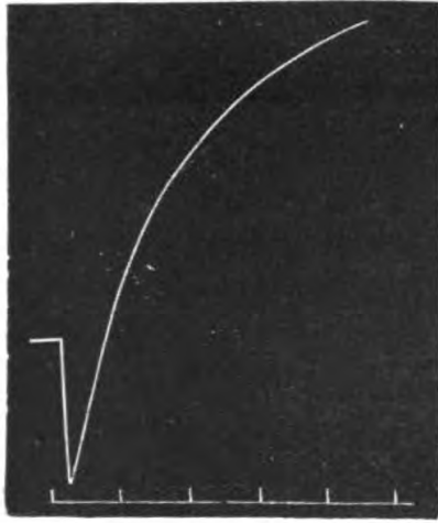
FIG. 220. Mechanical Response of Root of Bindweed to very strong Unilateral Stimulation applied at the Tip
