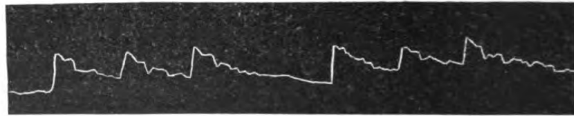
FIG. 121. Intermittent Human Pulse (Broadbent)
