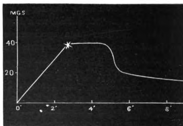
FIG. 165. Effect of Copper Sulphate Solution
