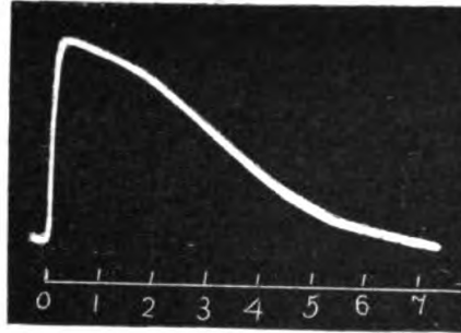
FIG. 15. Photographic Record of Response and Recovery of Mimosa , taken on a slowly moving drum. Record shows actual movement reduced to one-third.
