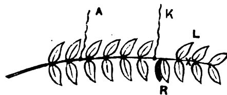
FIG. 103. 'Developing' Action of Kathode
