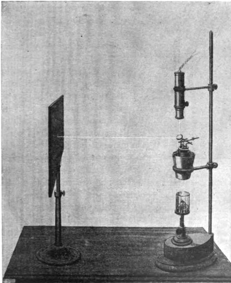
FIG. 84. The Morograph
