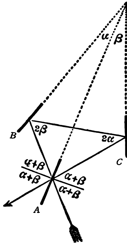
FIG. 7.—Plan of Interference Kaleidoscope with three mirrors.
