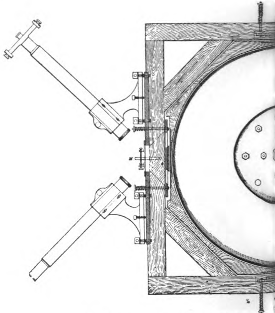
FIG. 19 Plan of optical frame with steel disk in position. G represents one of the panes of optical system shown, and part of the fixing of the four mirror frame, each mirror held by a brass plate which it is pressed by the spring-bolts shown.
