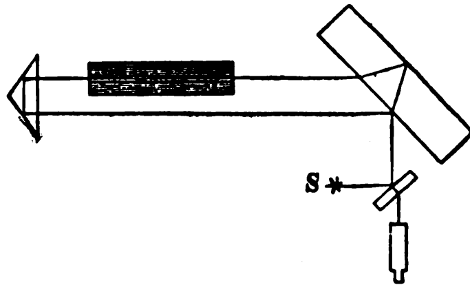
FIG. 9.—Arrangement of Mascart and Jamin.
