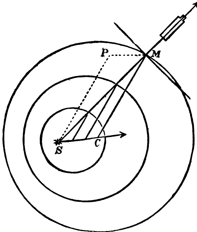
FIG. 5.—Successive Wave Fronts in a Moving Medium.
