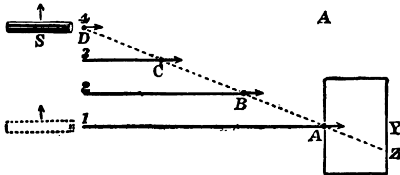
FIG. 2.—Waves or Disturbances without Momentum from a Moving Source.
