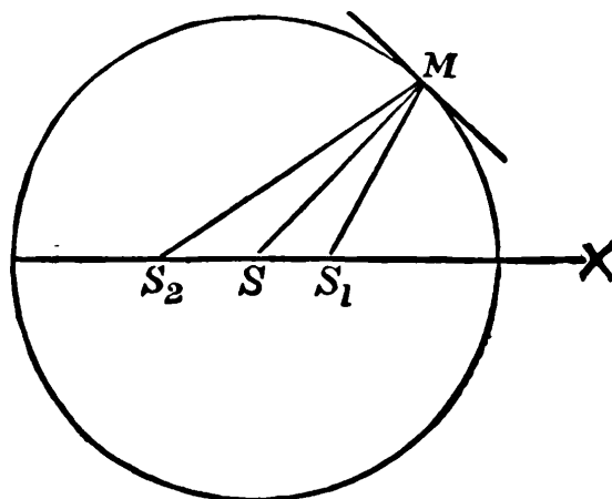
FIG. 6.—Normal Reflection in Moving Medium.
