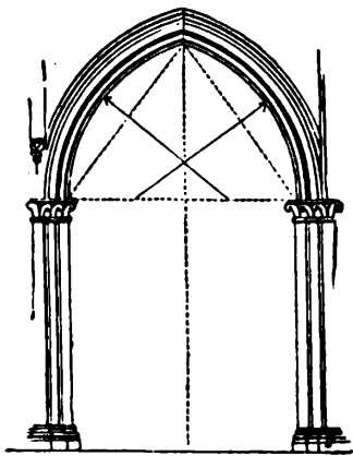
7. Obtuse Angle Arch.
