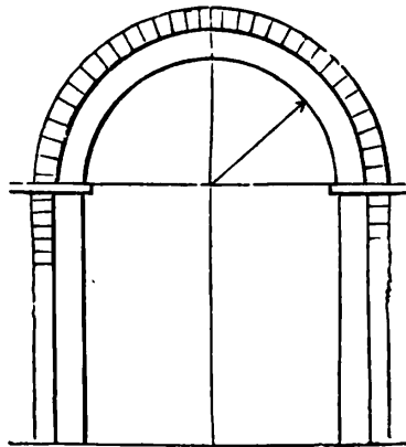
1. Semicircular Arch.
