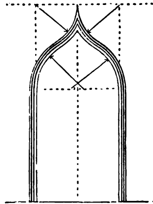
8. Ogee Arch.
