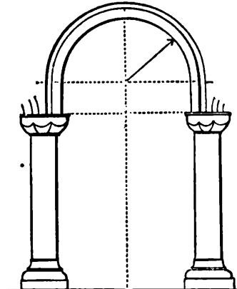
2. Stilted Arch.
