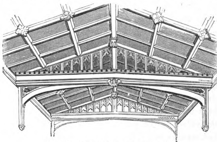
Roof, St. Mary's Church, Leicester.
