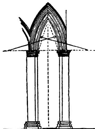
5. Lancet Arch.
