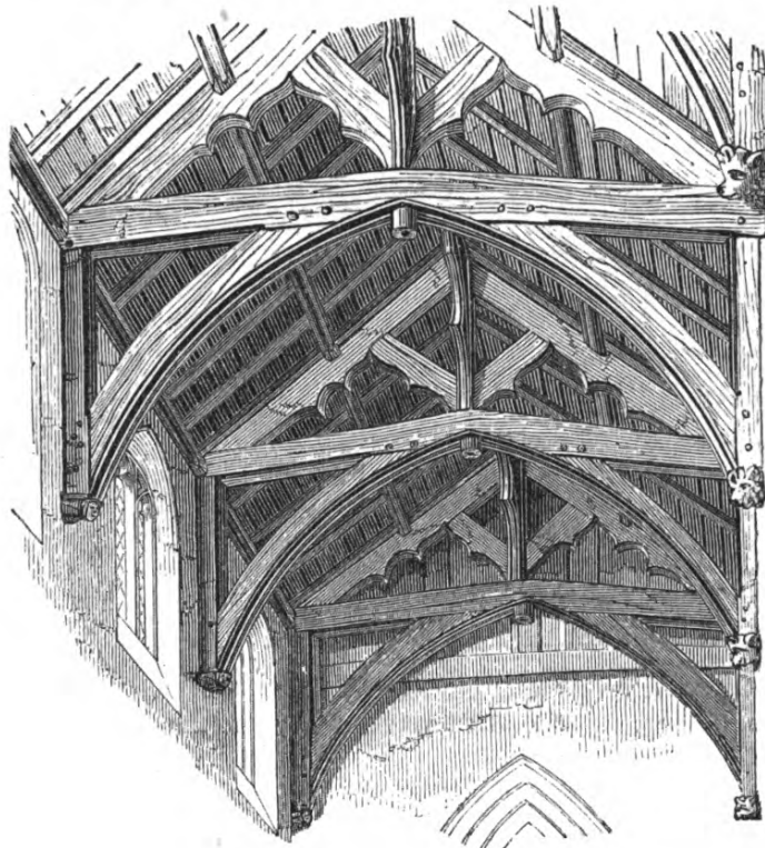
Roof, west end of Nave.
