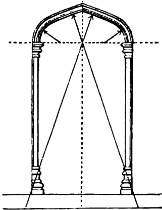
9. Tudor Arch.
